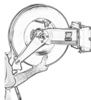
The insertion of the hose reel in the wall bracket is with quick disconnect coupling
